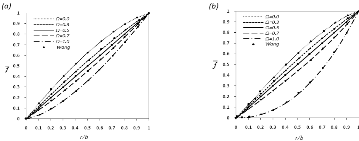
Fig. 3 Variations of dimensionless parameter of the stress function \bar{f} with respect to dimensionless parameter of radial coordinate r/b , (a): Linear taper; (b): Parabolic taper.
