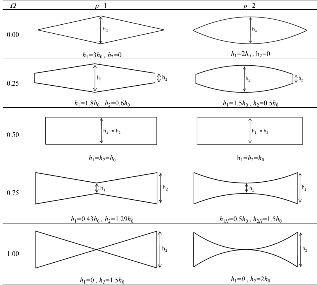
Fig. 2 Plate sections for various values of taper parameter \Omega and corresponding values of h_1 and h_2 .
