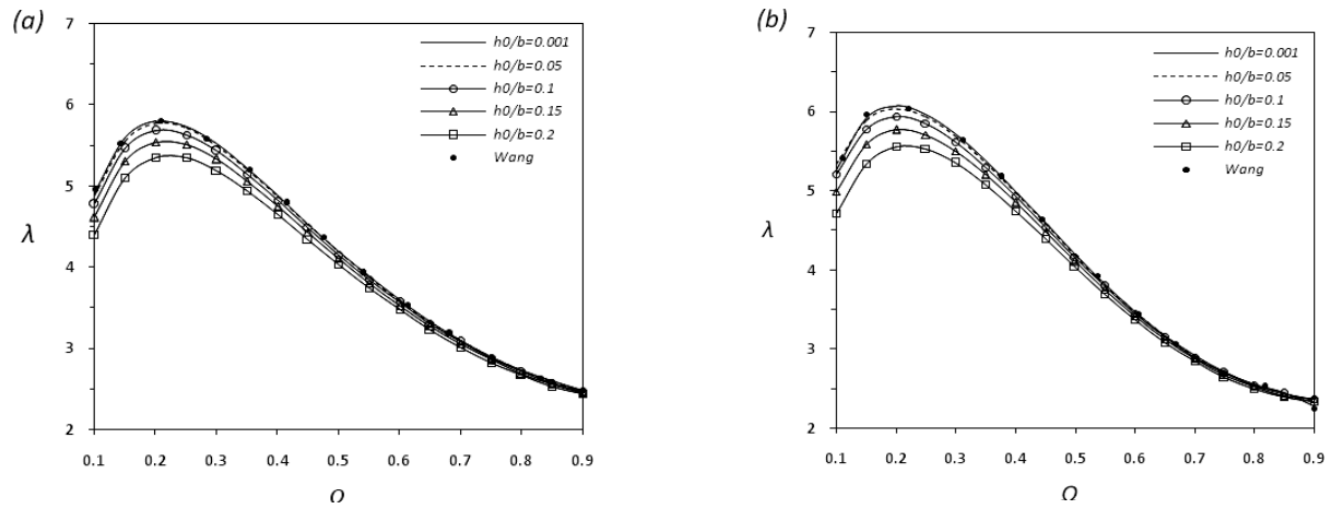
Fig. 5 Buckling load factor \lambda with respect to taper parameter \Omega for simply supported edge, (a): Linear taper; (b): Parabolic taper.
