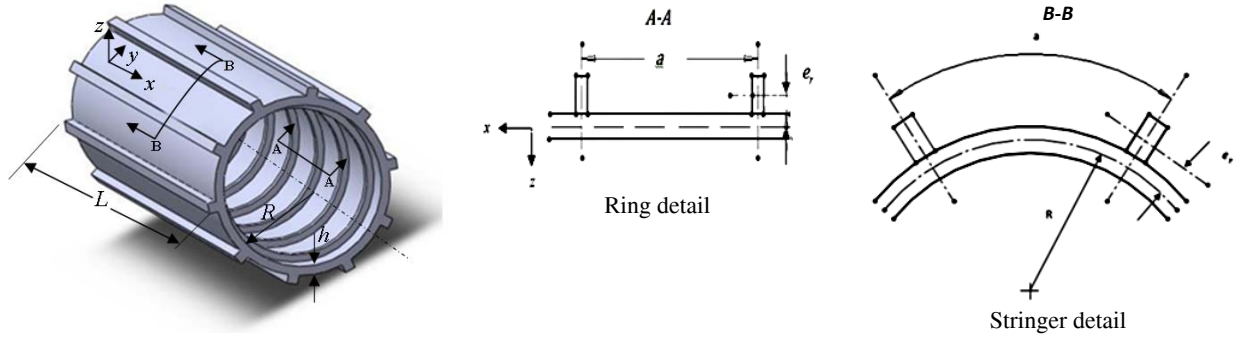
Fig. 1 Geometry and coordinate system of a stiffened cylindrical shell.
