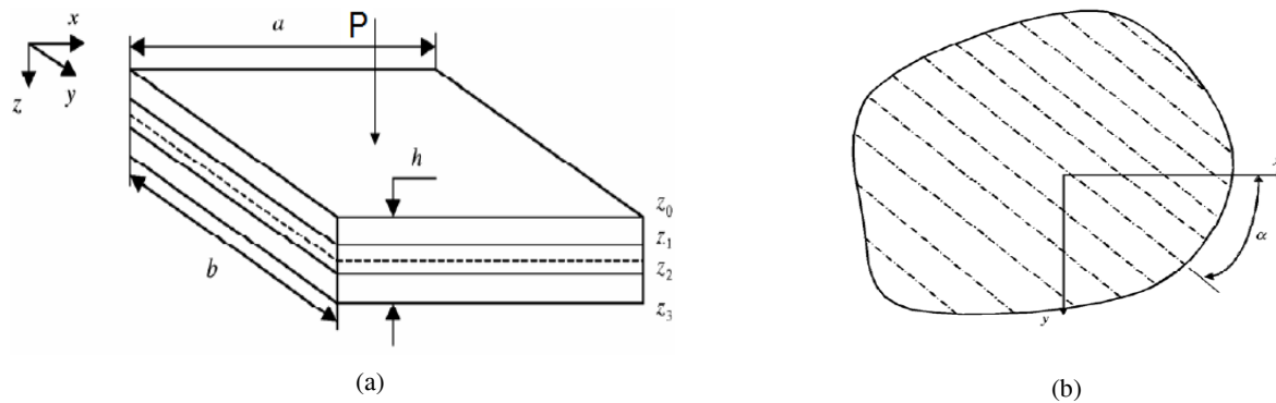
Fig.2 (a) A laminated plate under transverse loading. (b) Fiber orientation in a laminate.
