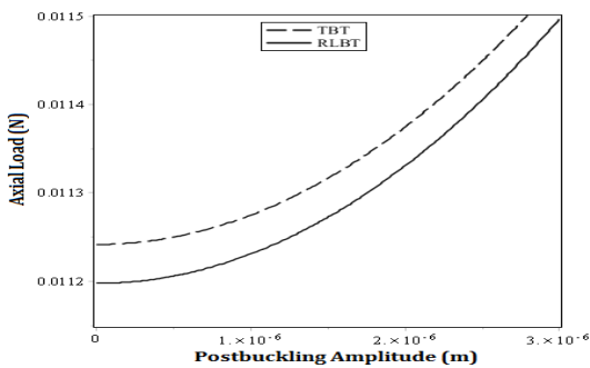
Fig.4 Comparison of the static postbuckling response of the TBT and RLBT with h/\xi = 1 .
