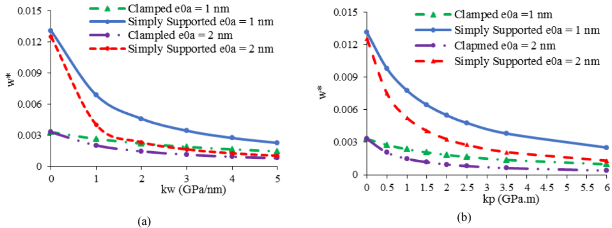
Fig.11 Dimensionless deflection versus (a) Winkler stiffness foundation. (b) Pasternak stiffness foundation.
